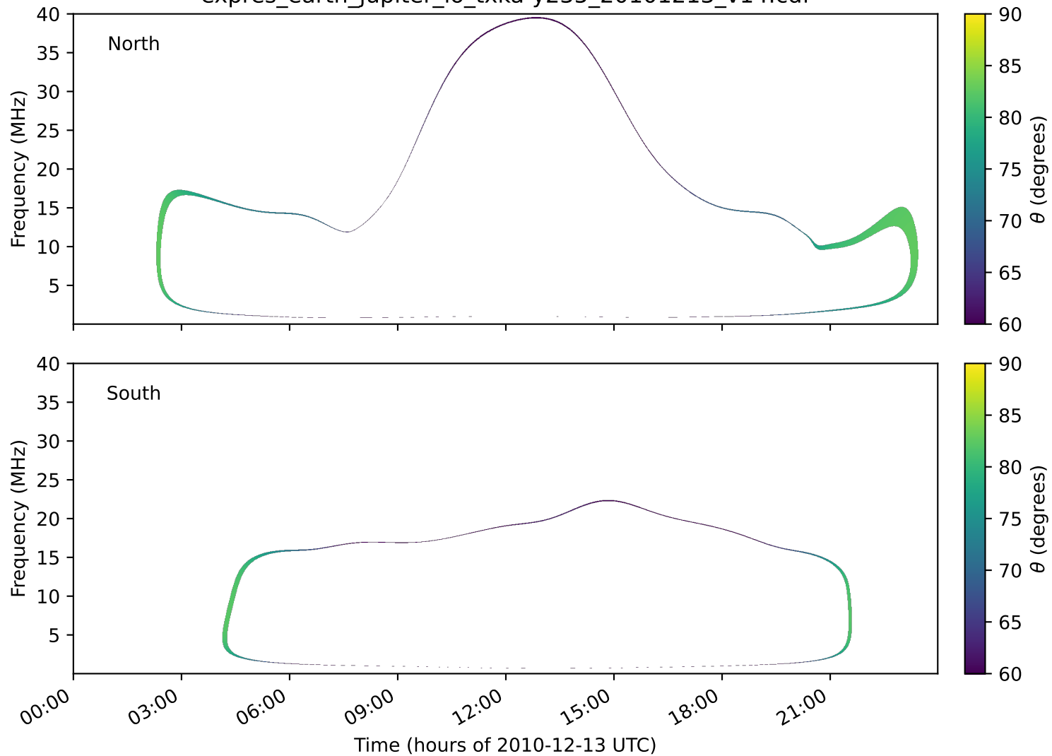
expres_earth_jupiter_io_txka-y235_20101213_v14.cdf
