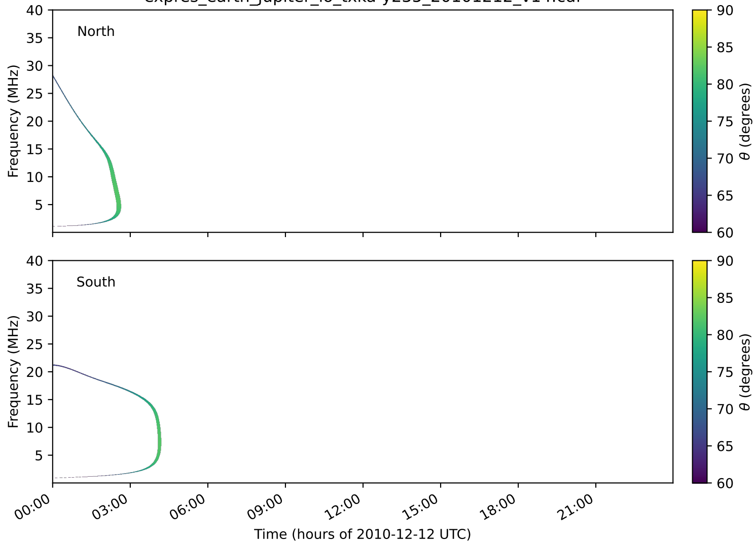
expres_earth_jupiter_io_txka-y235_20101212_v14.cdf
