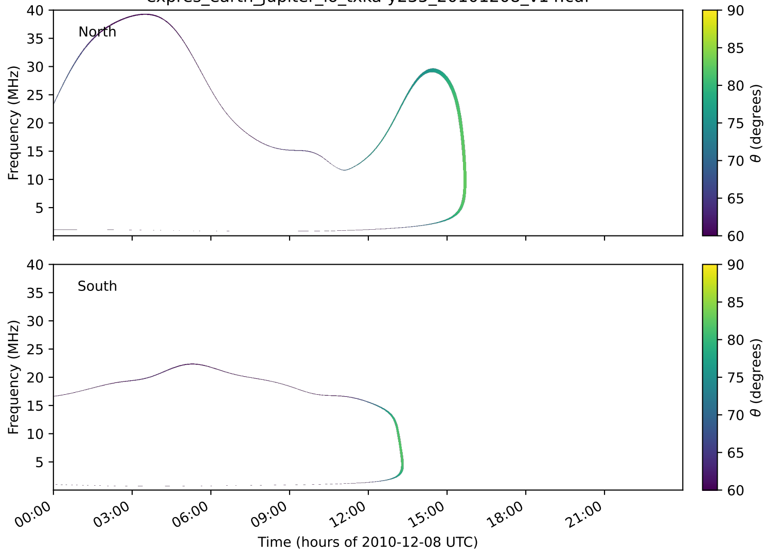
expres_earth_jupiter_io_txka-y235_20101208_v14.cdf
