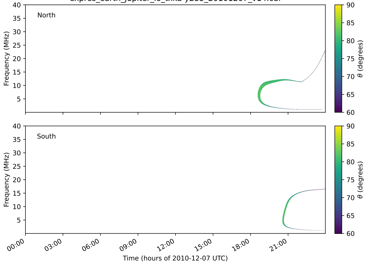
expres_earth_jupiter_io_txka-y235_20101207_v14.cdf
