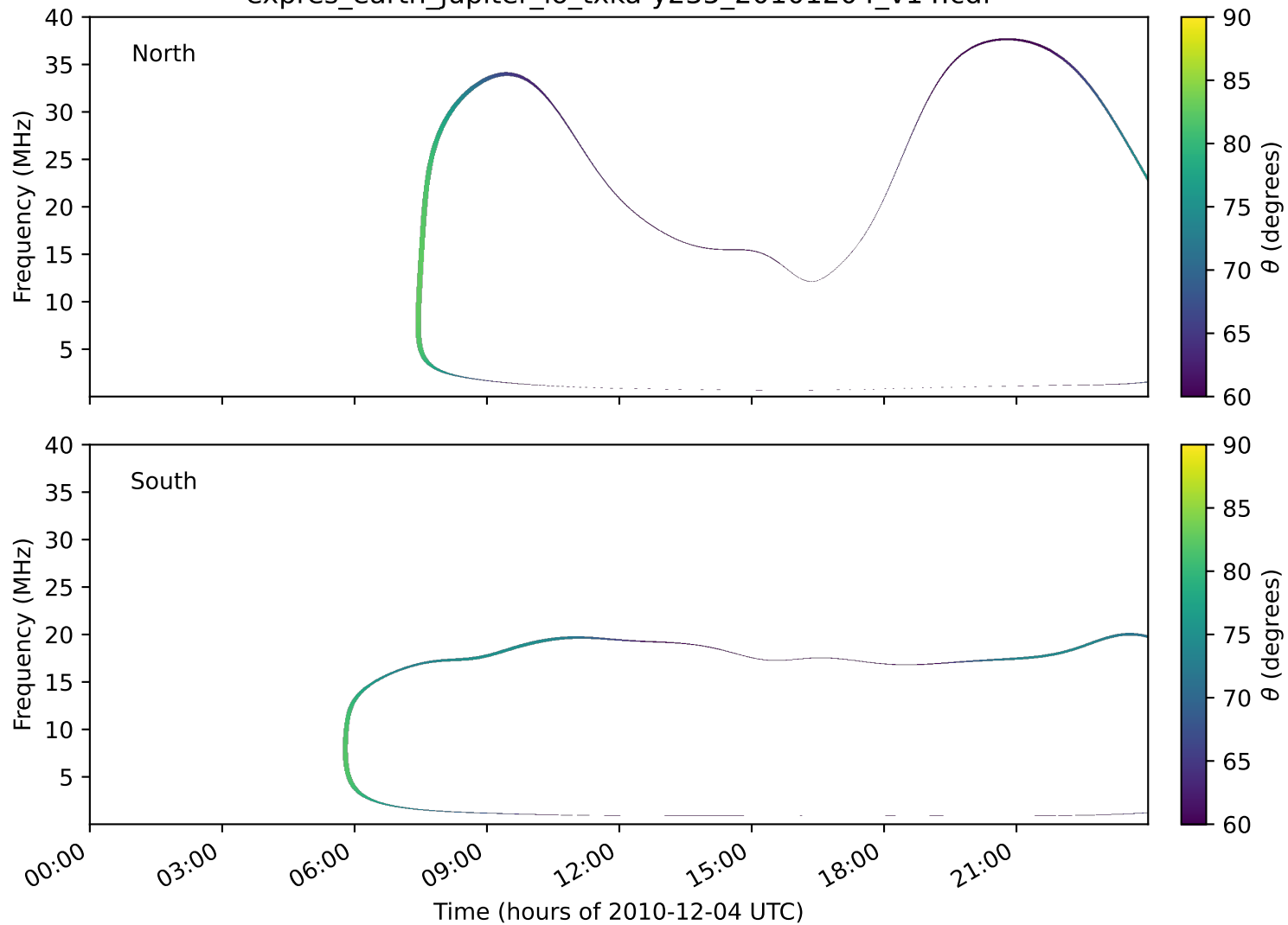
expres_earth_jupiter_io_txka-y235_20101204_v14.cdf
