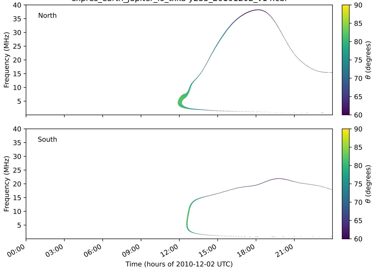
expres_earth_jupiter_io_txka-y235_20101202_v14.cdf
