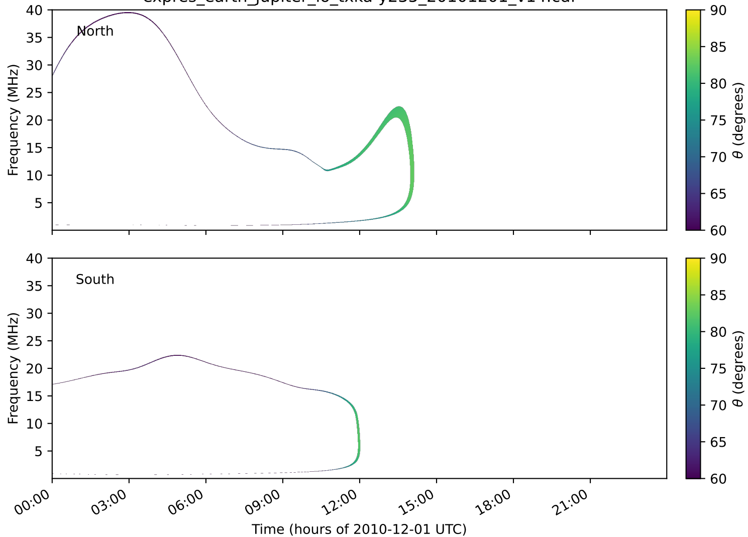
expres_earth_jupiter_io_txka-y235_20101201_v14.cdf
