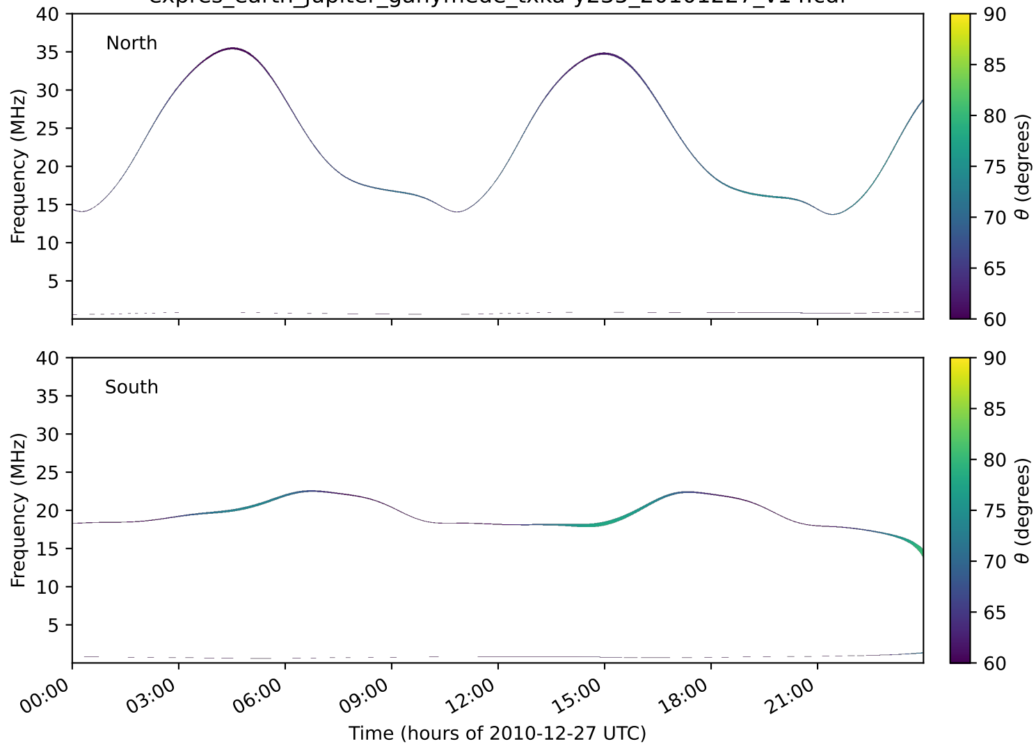
expres_earth_jupiter_ganymede_txka-y235_20101227_v14.cdf
