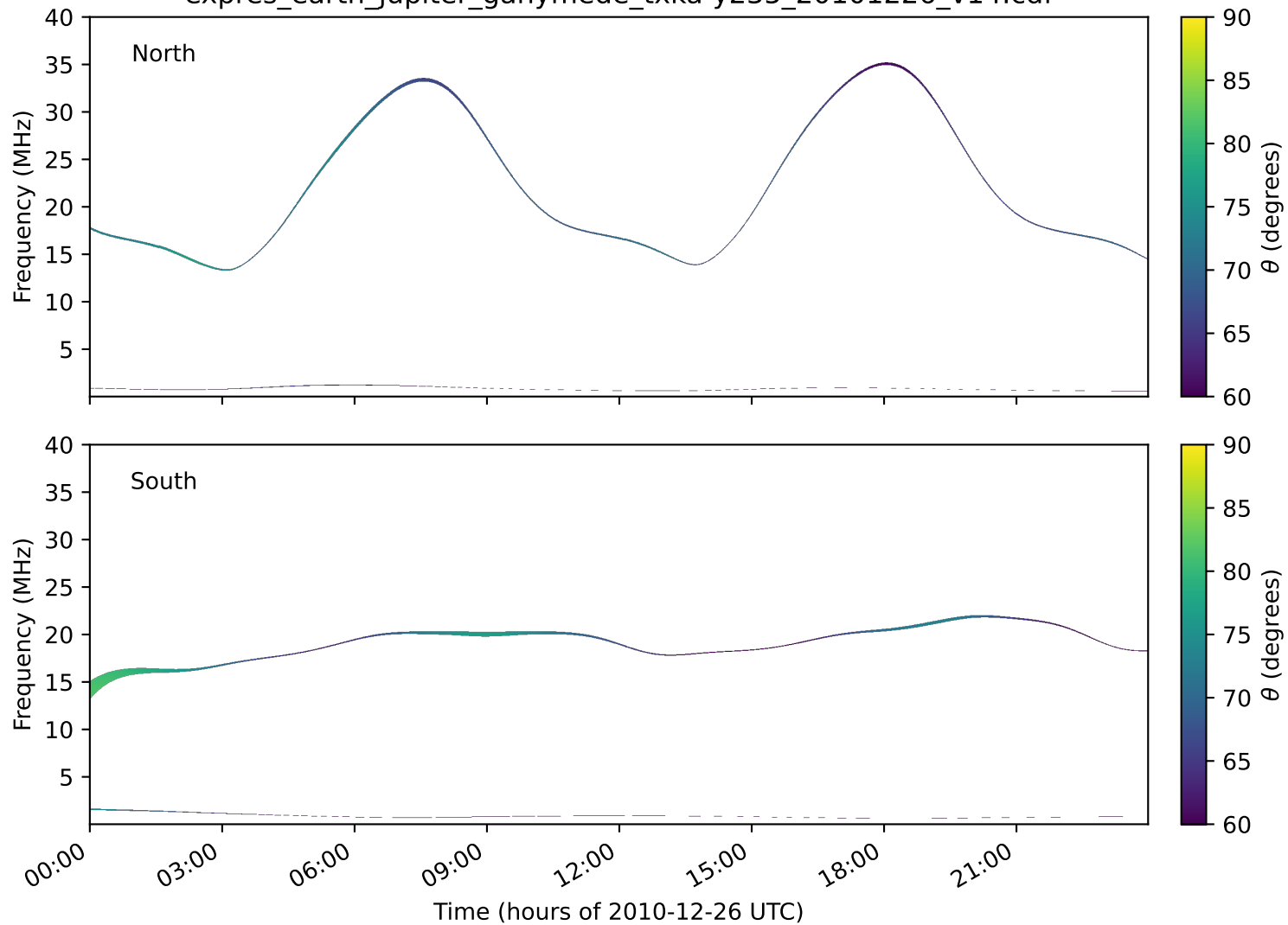
expres_earth_jupiter_ganymede_txka-y235_20101226_v14.cdf
