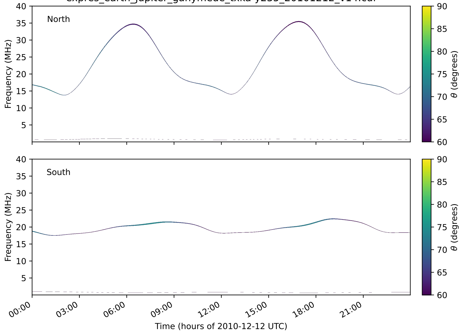
expres_earth_jupiter_ganymede_txka-y235_20101212_v14.cdf
