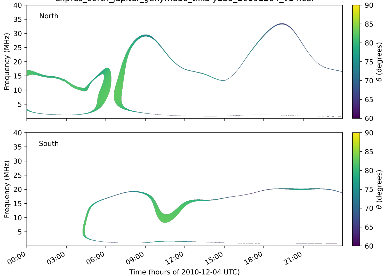
expres_earth_jupiter_ganymede_txka-y235_20101204_v14.cdf
