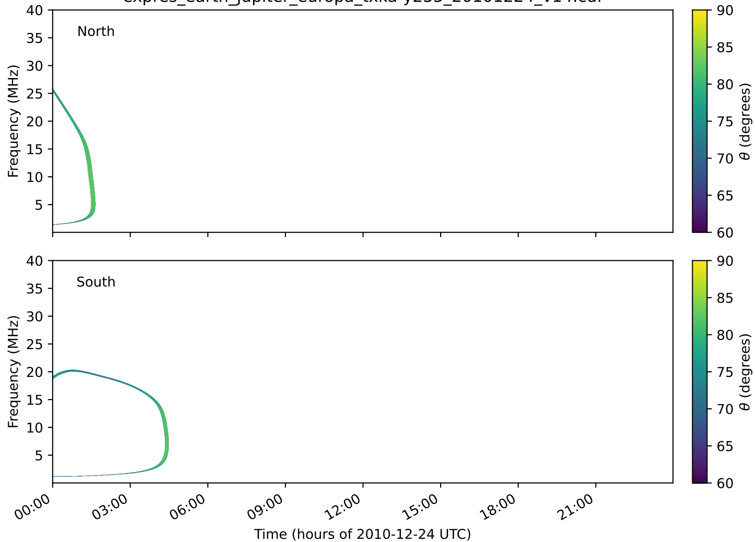
expres_earth_jupiter_europa_txka-y235_20101224_v14.cdf
