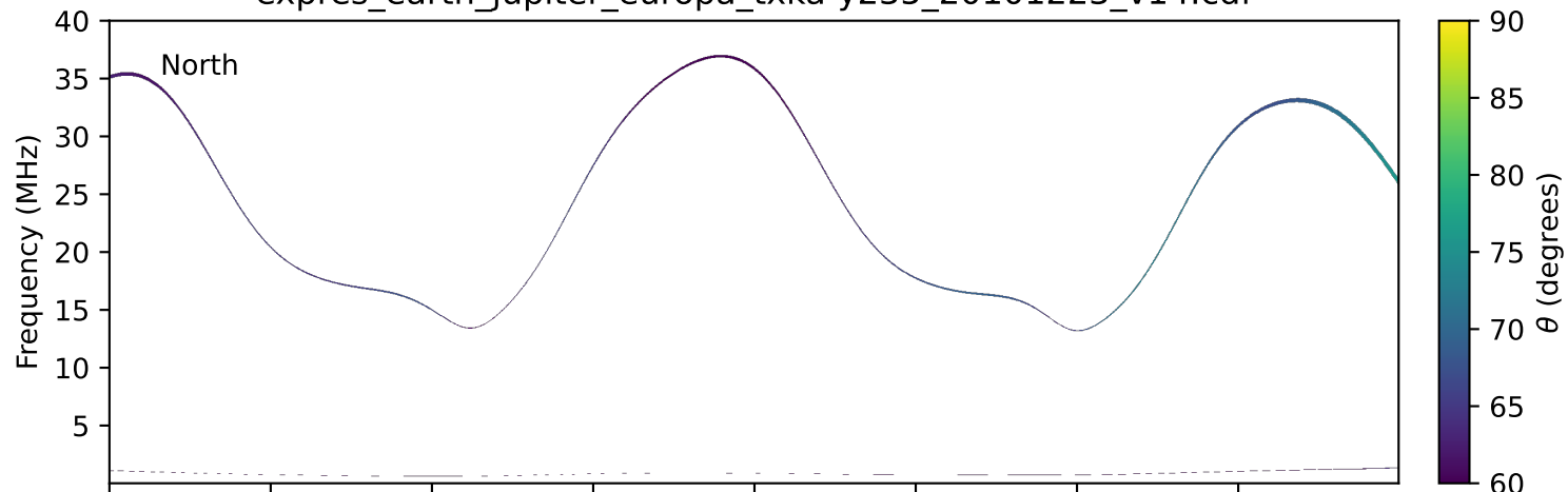
expres_earth_jupiter_europa_txka-y235_20101223_v14.cdf
