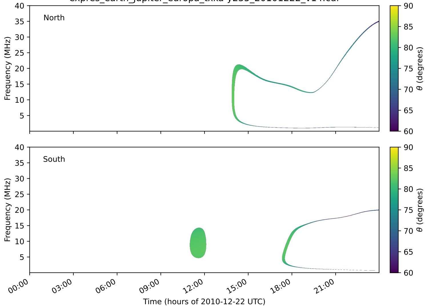
expres_earth_jupiter_europa_txka-y235_20101222_v14.cdf
