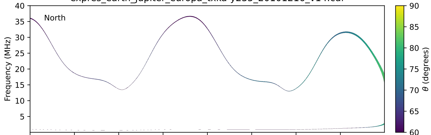
expres_earth_jupiter_europa_txka-y235_20101216_v14.cdf
