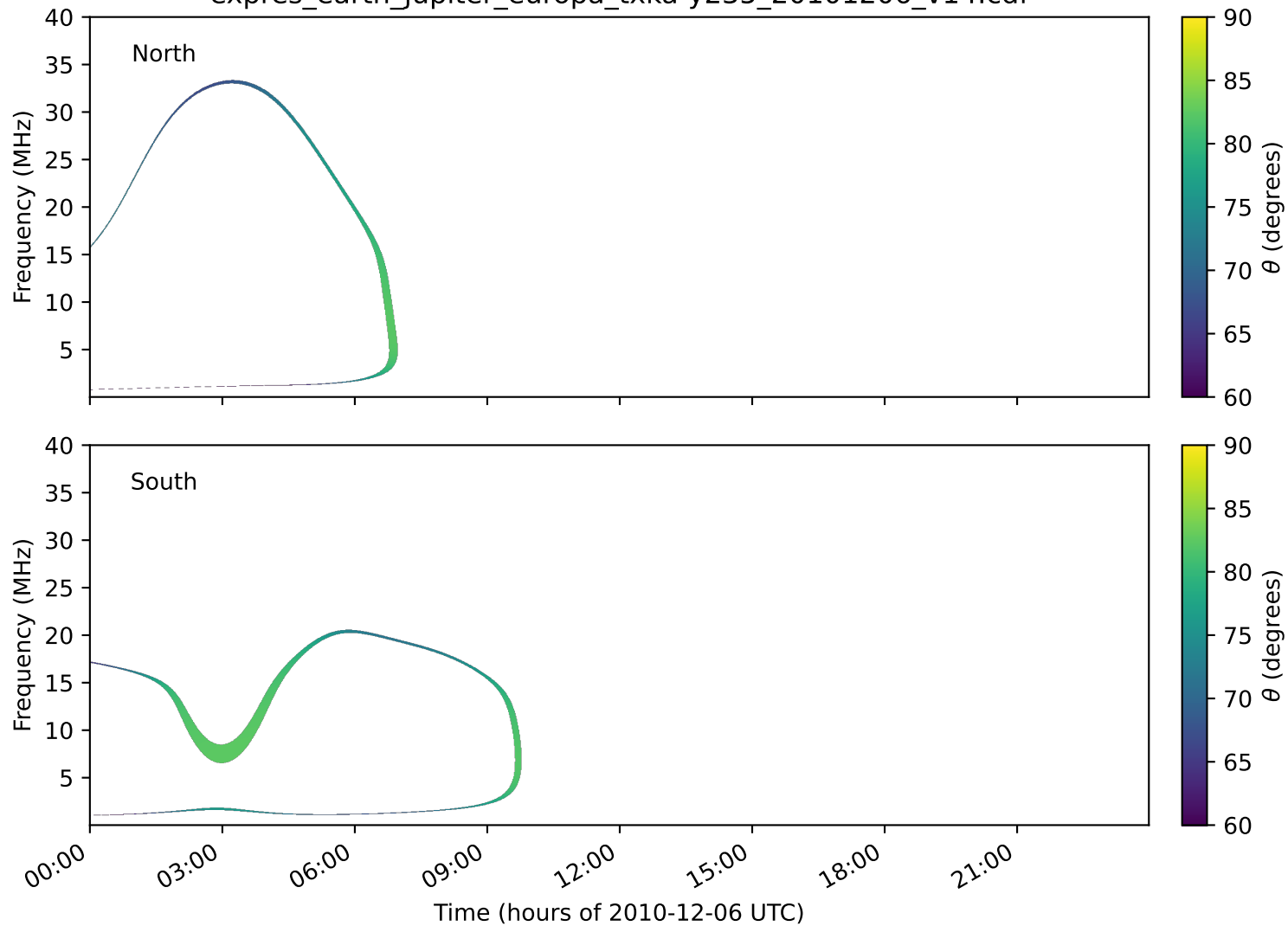
expres_earth_jupiter_europa_txka-y235_20101206_v14.cdf
