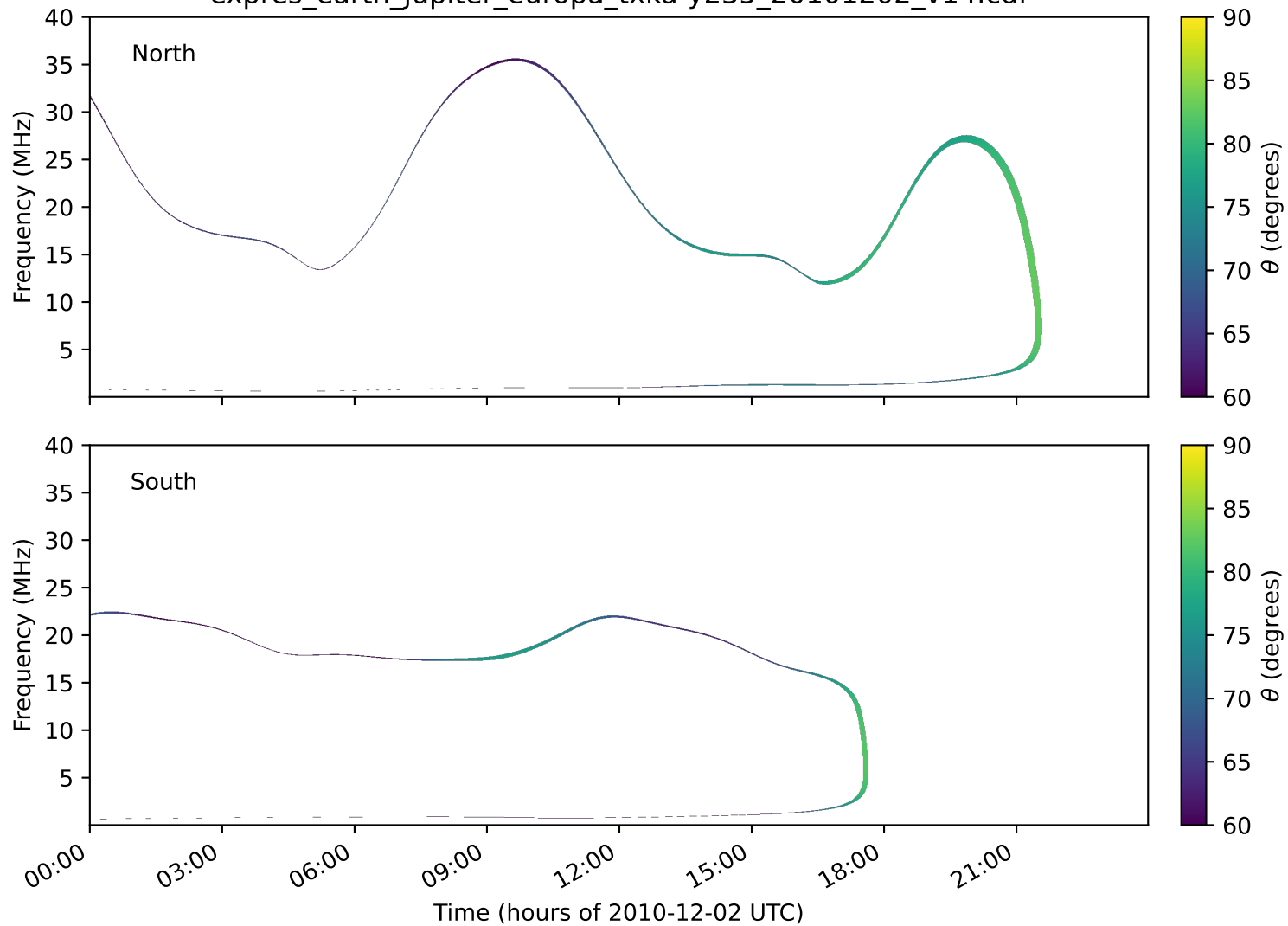
expres_earth_jupiter_europa_txka-y235_20101202_v14.cdf
