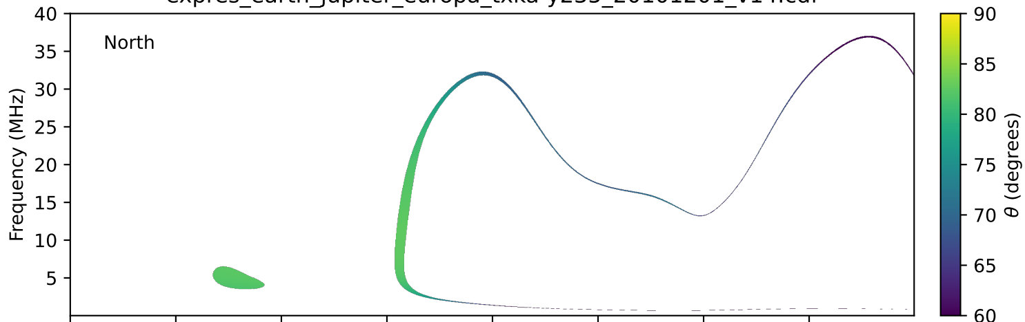
expres_earth_jupiter_europa_txka-y235_20101201_v14.cdf
