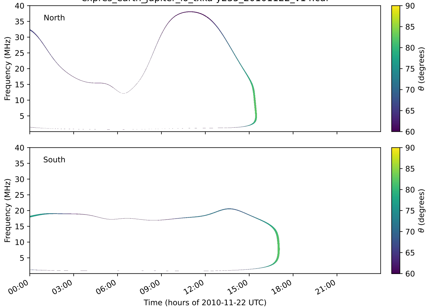
expres_earth_jupiter_io_txka-y235_20101122_v14.cdf
