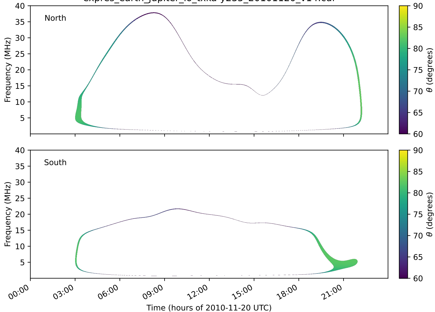
expres_earth_jupiter_io_txka-y235_20101120_v14.cdf
