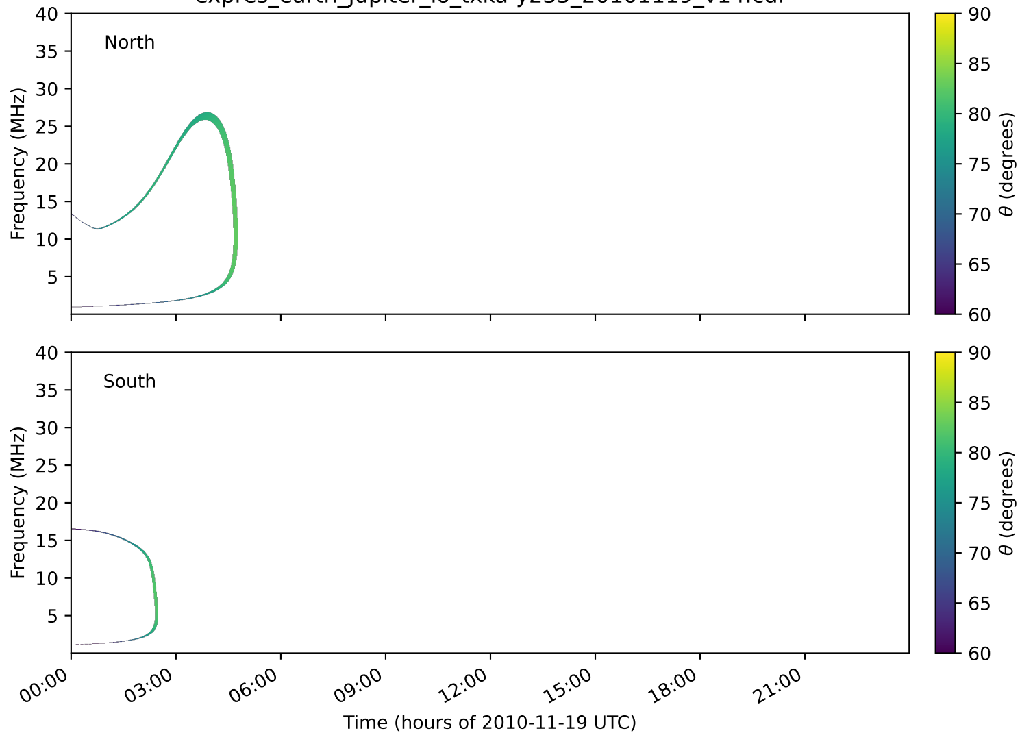
expres_earth_jupiter_io_txka-y235_20101119_v14.cdf
