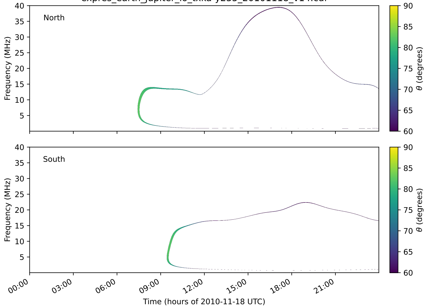
expres_earth_jupiter_io_txka-y235_20101118_v14.cdf
