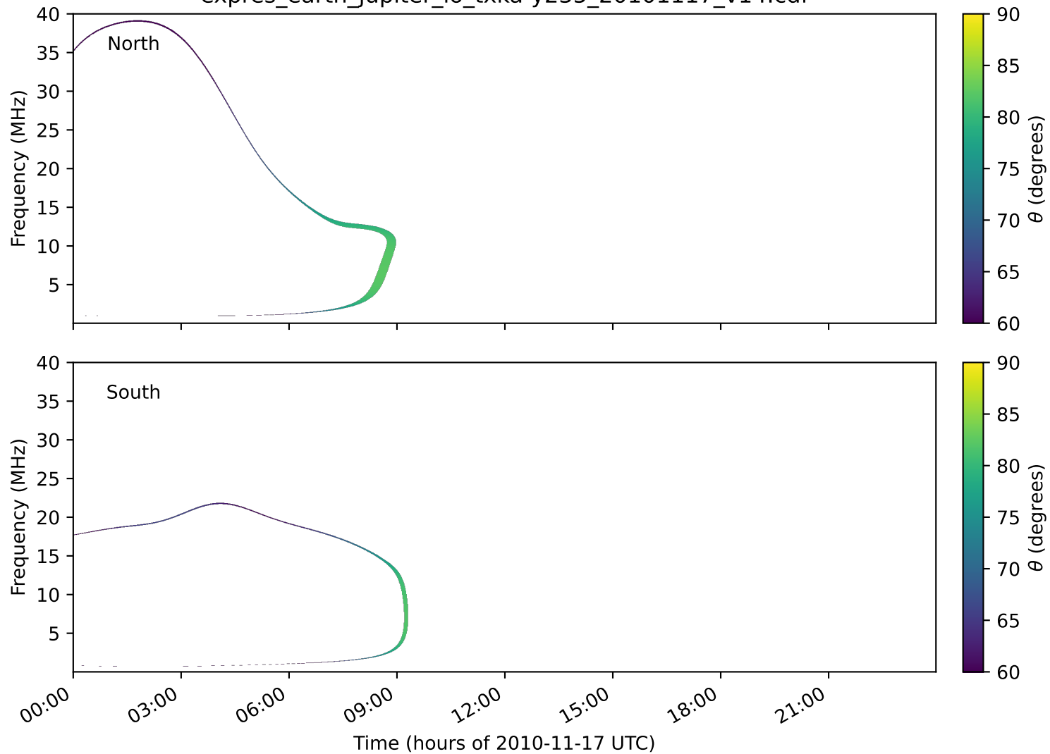
expres_earth_jupiter_io_txka-y235_20101117_v14.cdf
