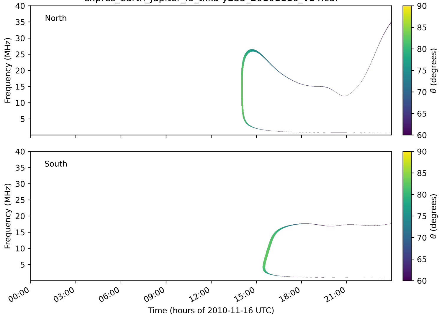
expres_earth_jupiter_io_txka-y235_20101116_v14.cdf
