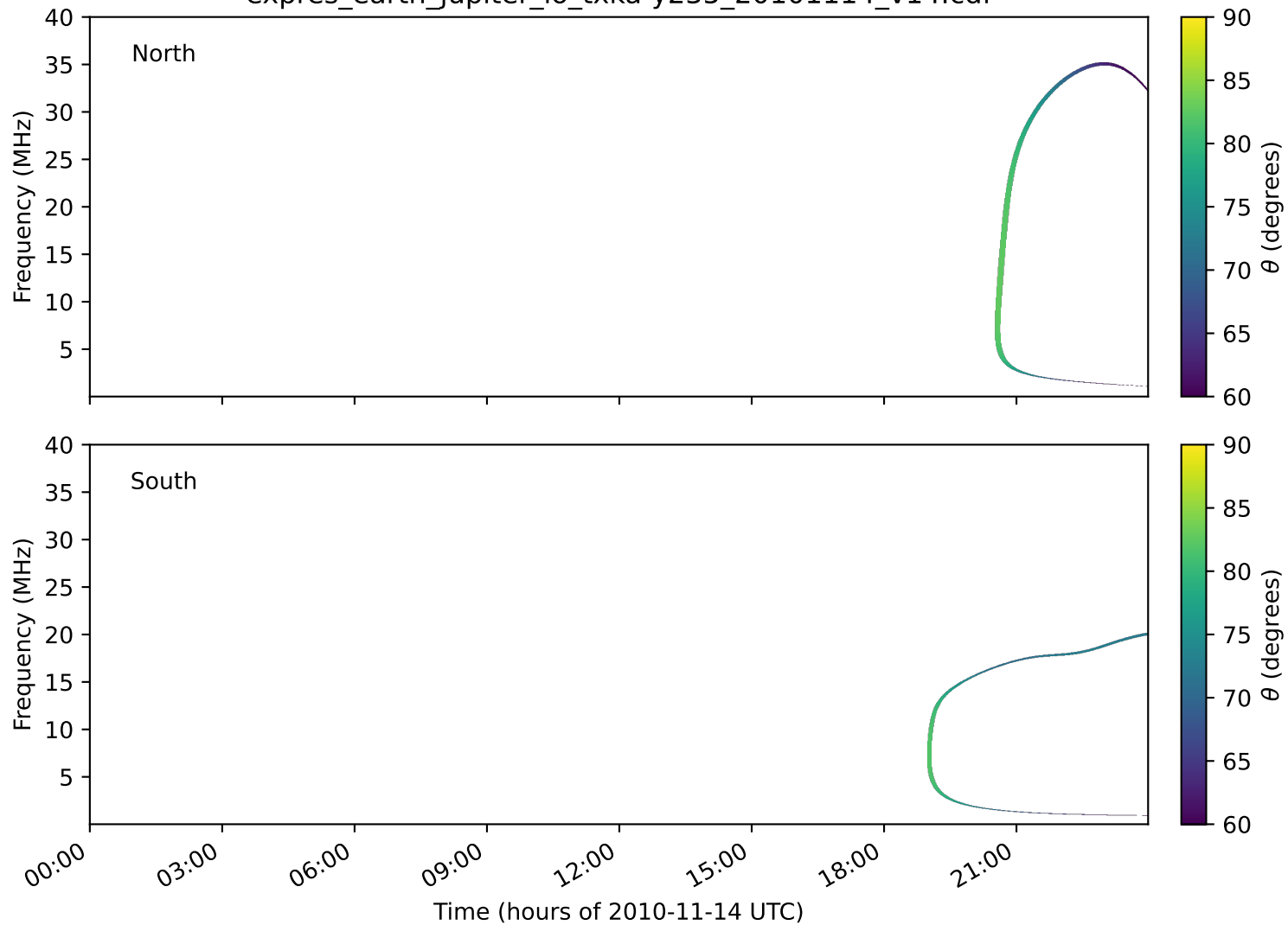
expres_earth_jupiter_io_txka-y235_20101114_v14.cdf
