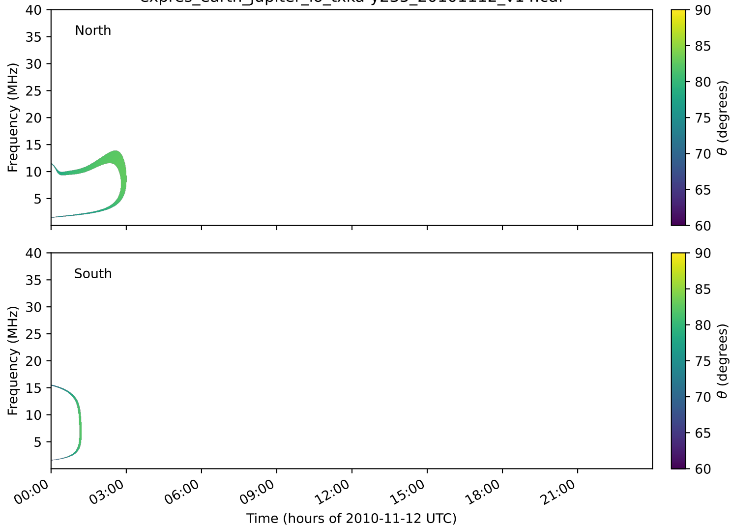
expres_earth_jupiter_io_txka-y235_20101112_v14.cdf
