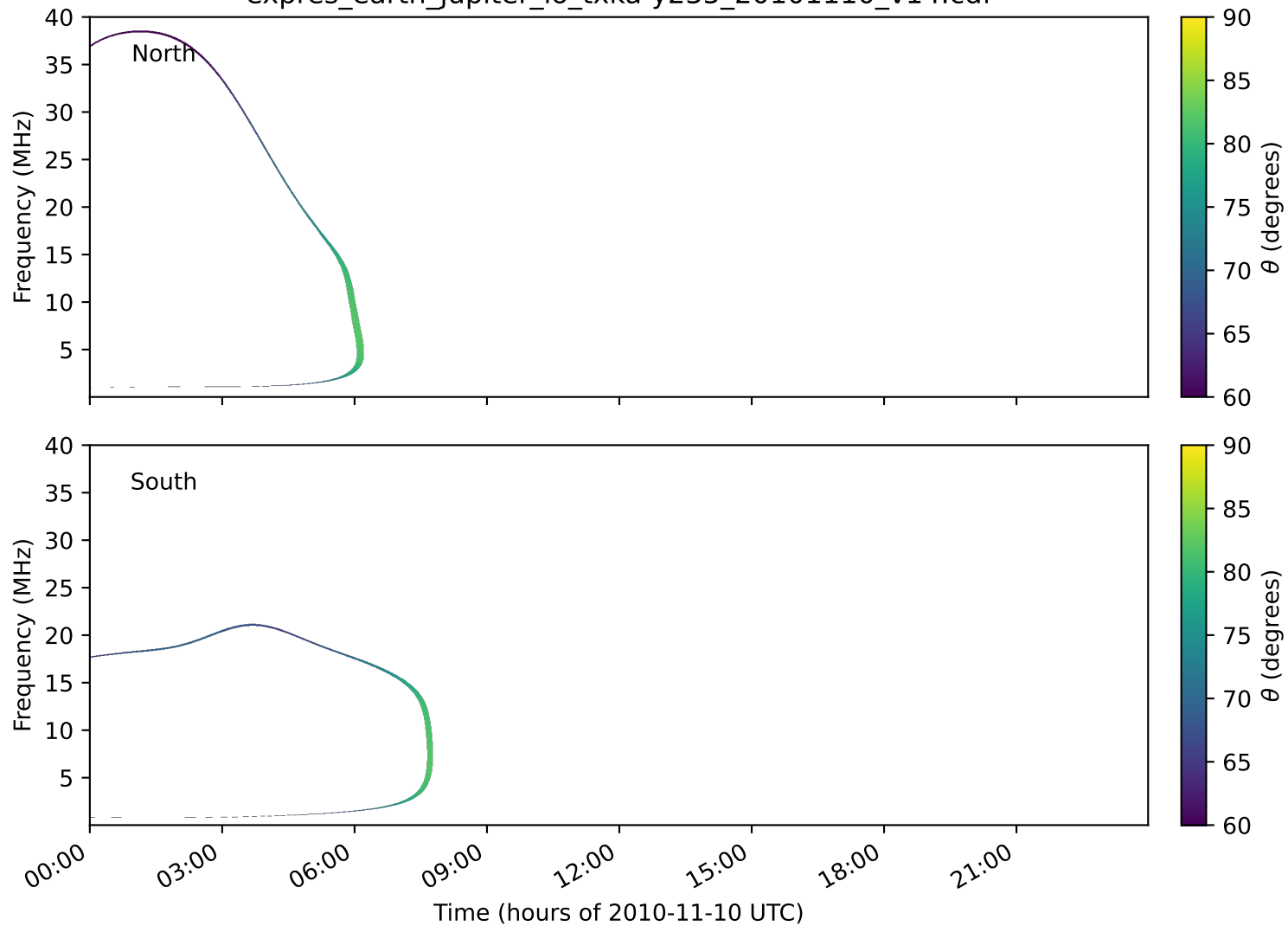
expres_earth_jupiter_io_txka-y235_20101110_v14.cdf
