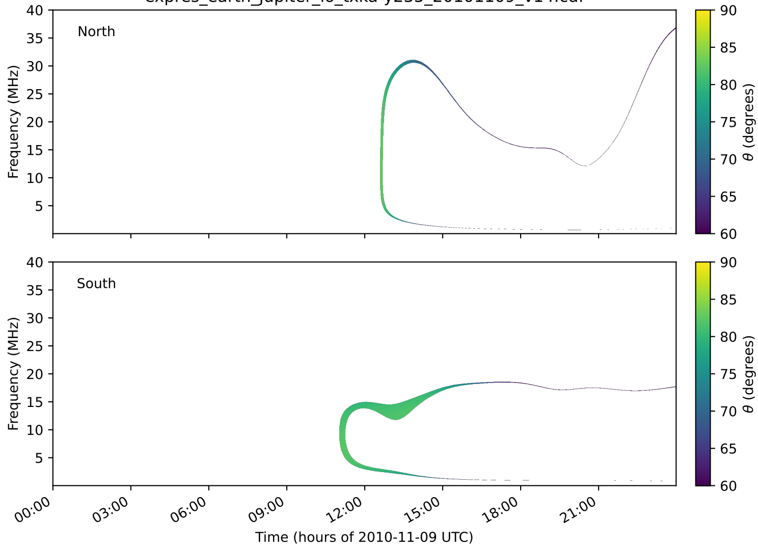
expres_earth_jupiter_io_txka-y235_20101109_v14.cdf
