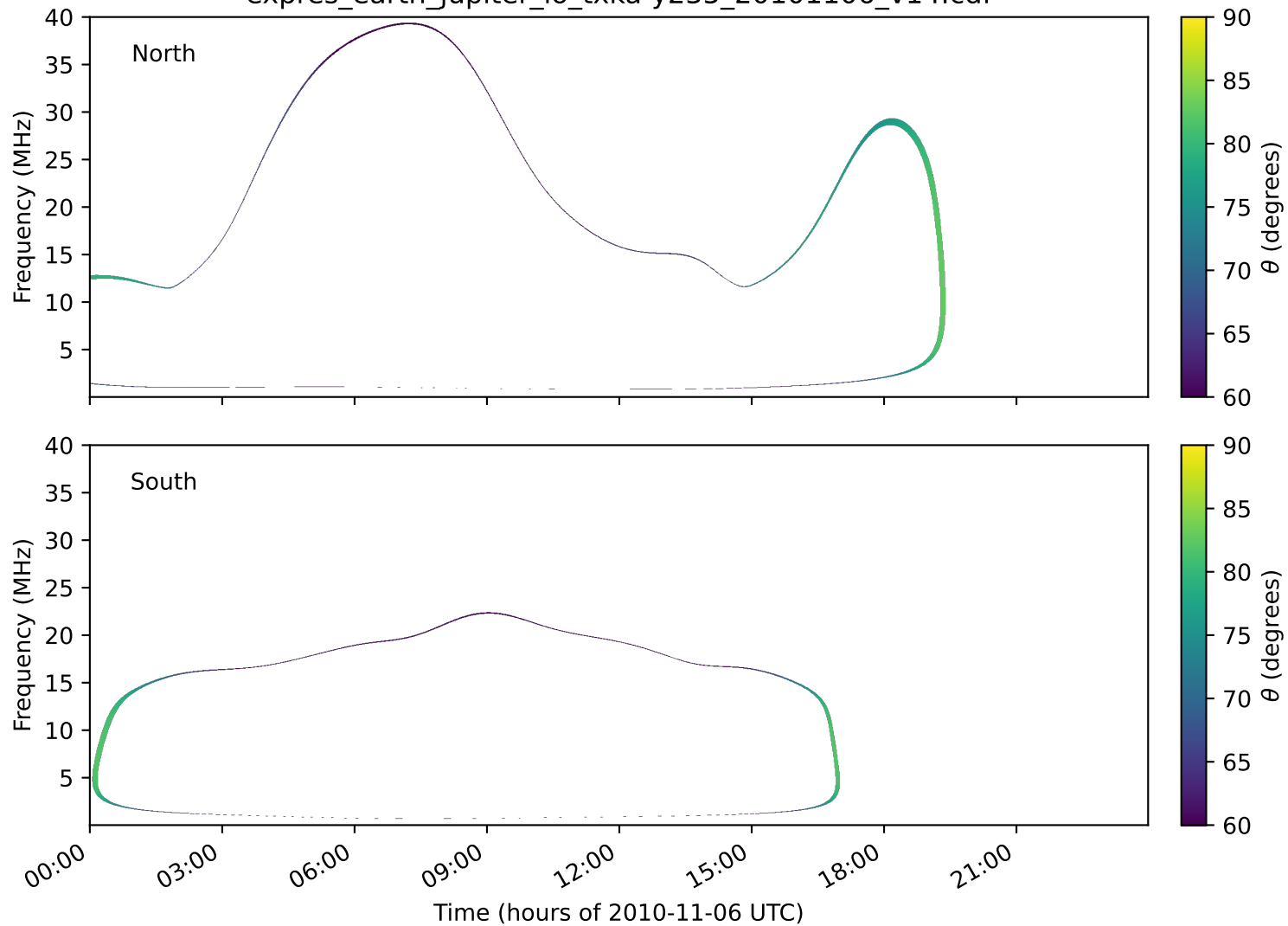
expres_earth_jupiter_io_txka-y235_20101106_v14.cdf
