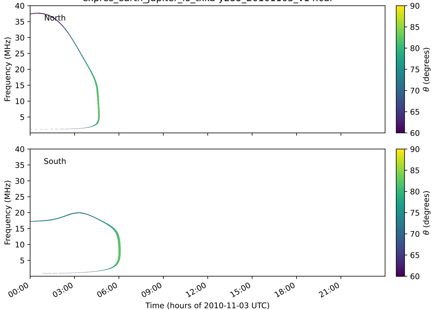
expres_earth_jupiter_io_txka-y235_20101103_v14.cdf
