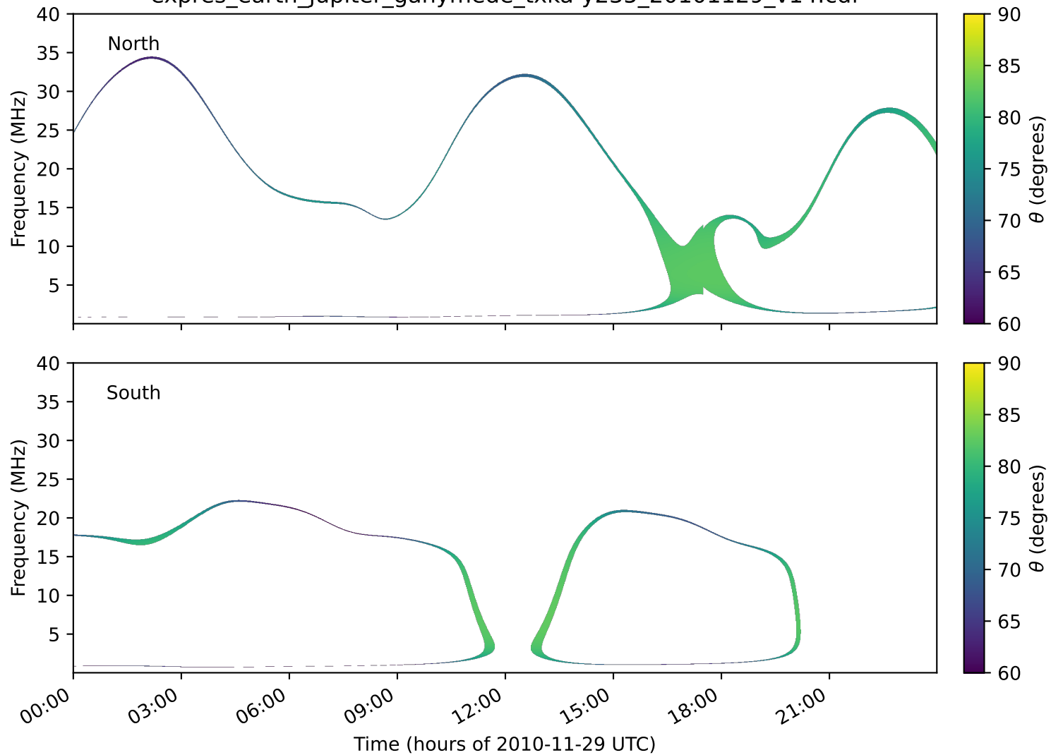
expres_earth_jupiter_ganymede_txka-y235_20101129_v14.cdf
