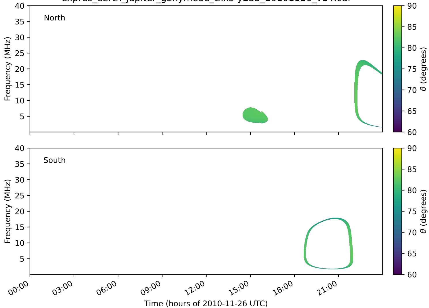
expres_earth_jupiter_ganymede_txka-y235_20101126_v14.cdf
