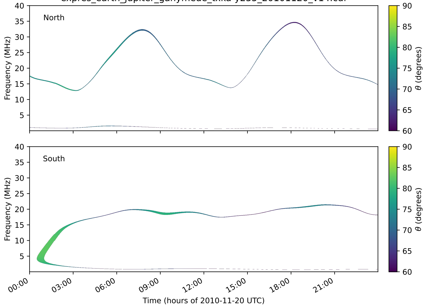
expres_earth_jupiter_ganymede_txka-y235_20101120_v14.cdf
