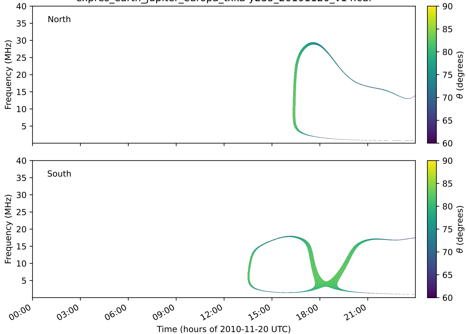
expres_earth_jupiter_europa_txka-y235_20101120_v14.cdf
