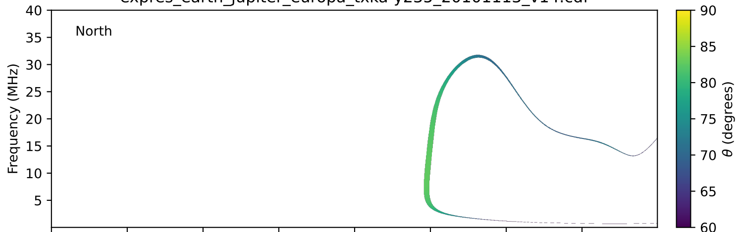
expres_earth_jupiter_europa_txka-y235_20101113_v14.cdf
