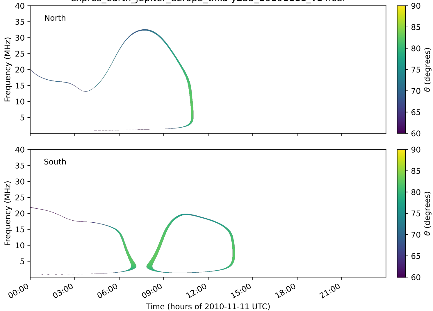
expres_earth_jupiter_europa_txka-y235_20101111_v14.cdf
