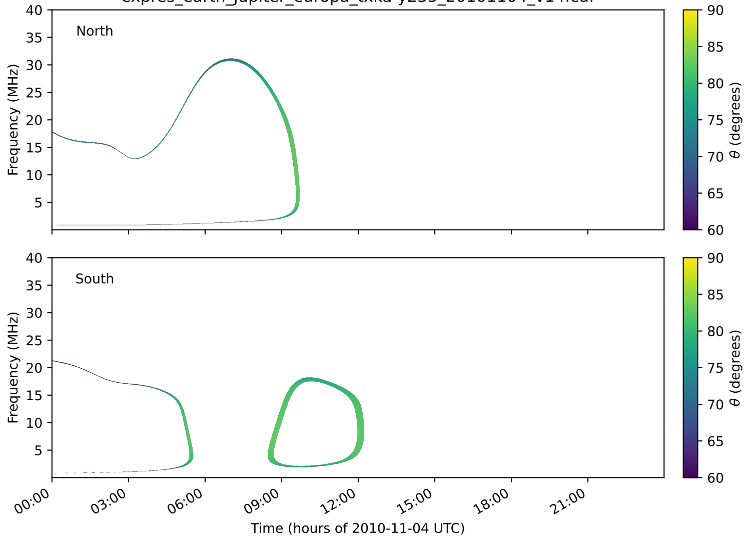
expres_earth_jupiter_europa_txka-y235_20101104_v14.cdf
