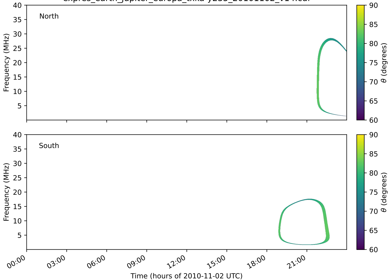
expres_earth_jupiter_europa_txka-y235_20101102_v14.cdf
