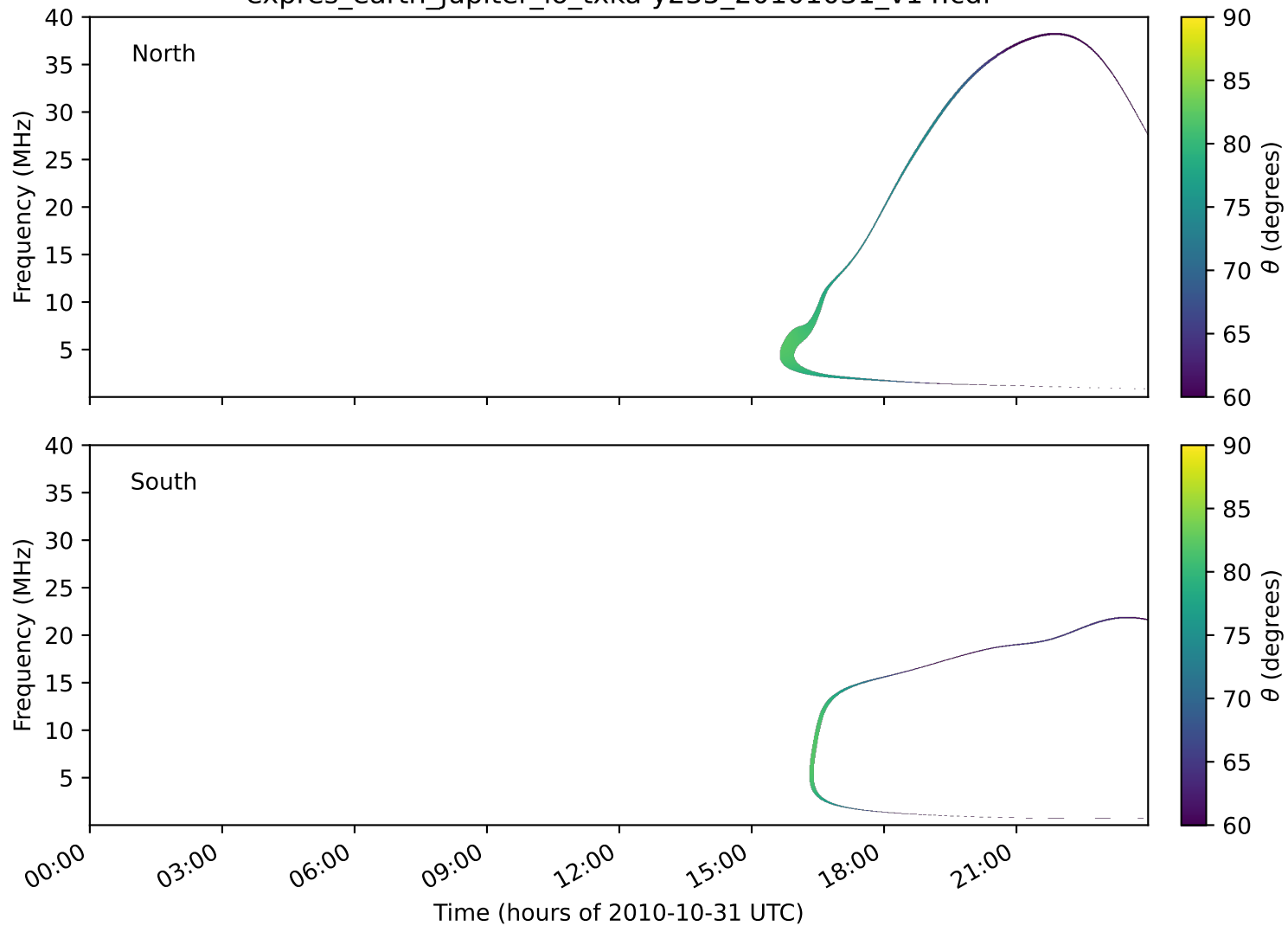
expres_earth_jupiter_io_txka-y235_20101031_v14.cdf
