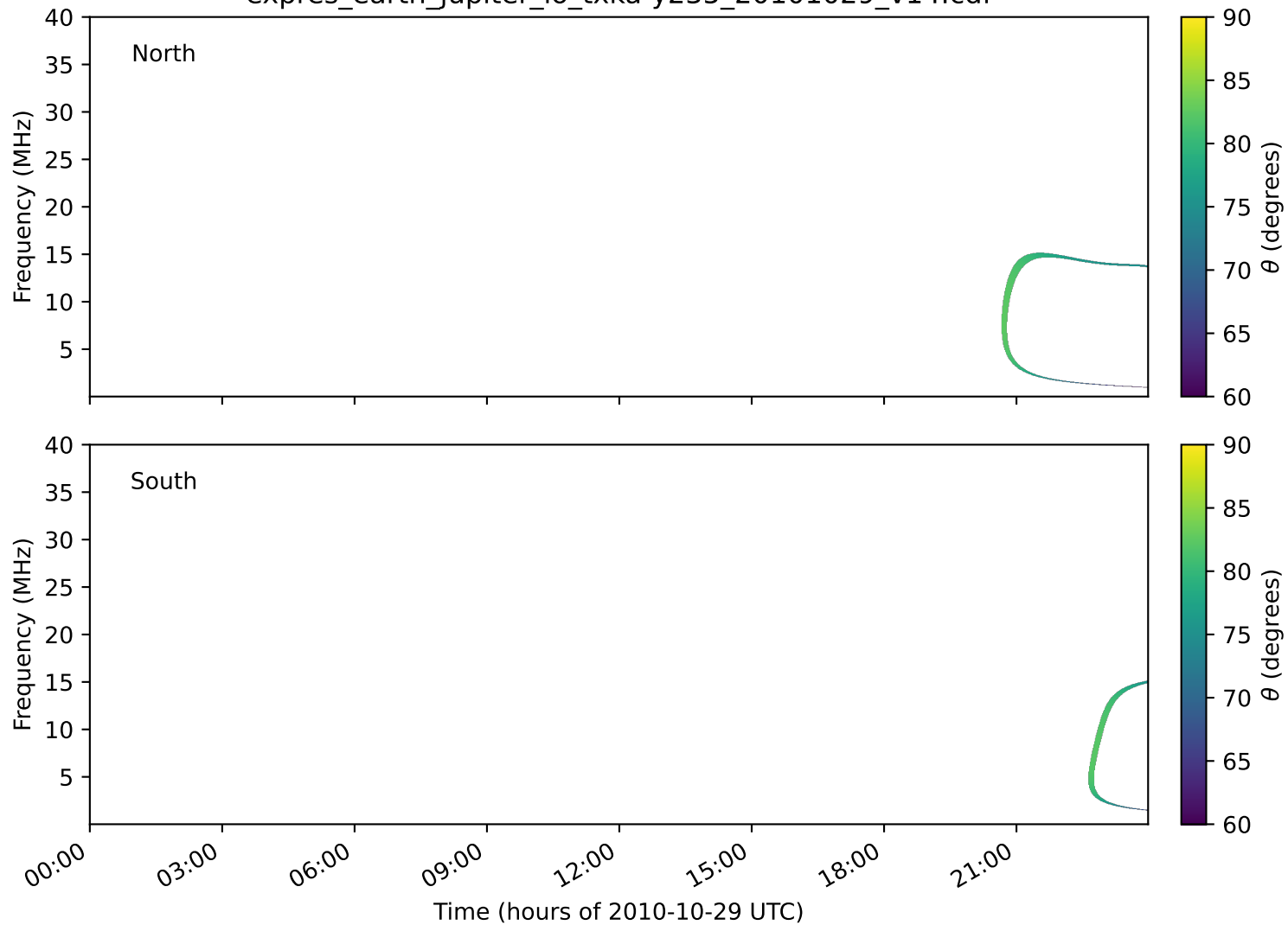
expres_earth_jupiter_io_txka-y235_20101029_v14.cdf
