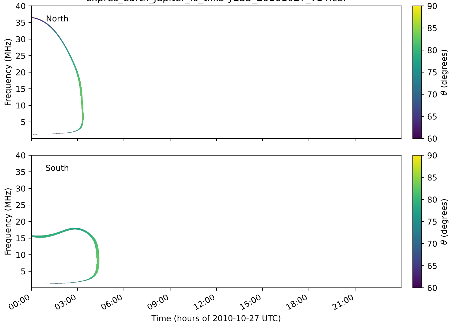
expres_earth_jupiter_io_txka-y235_20101027_v14.cdf
