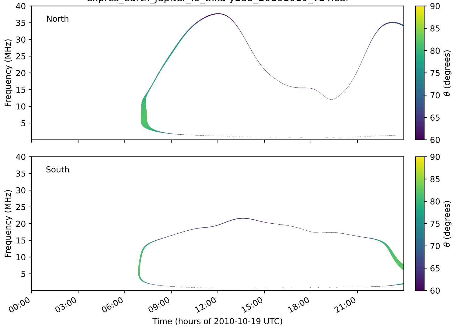
expres_earth_jupiter_io_txka-y235_20101019_v14.cdf
