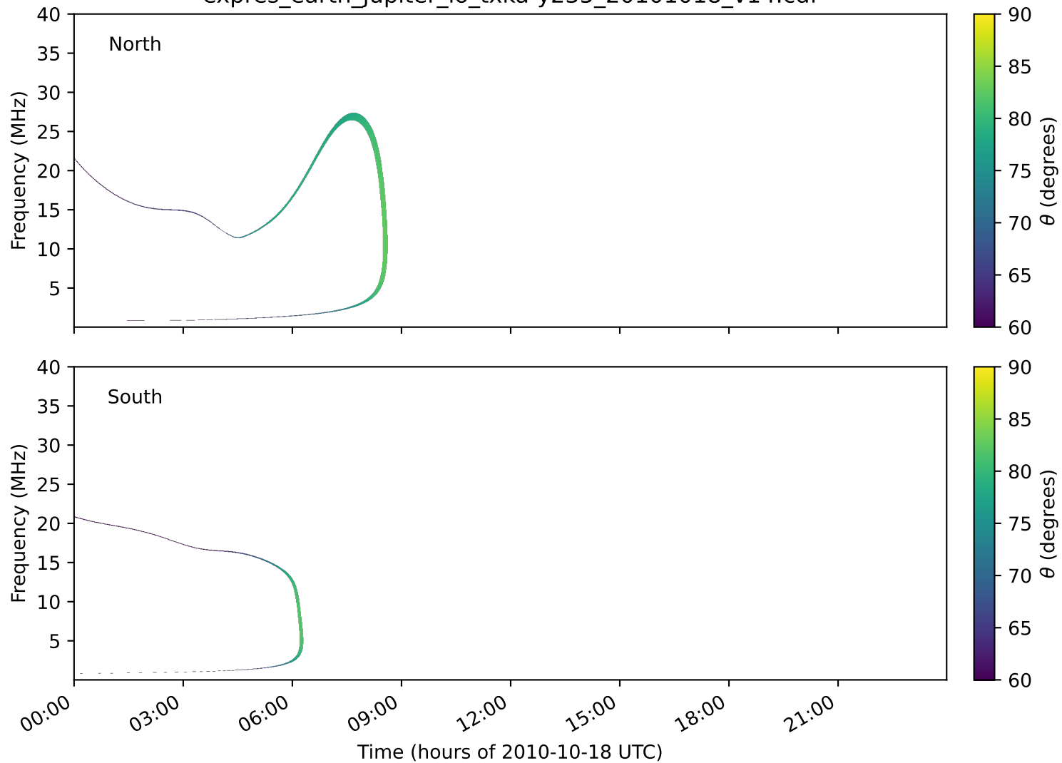
expres_earth_jupiter_io_txka-y235_20101018_v14.cdf
