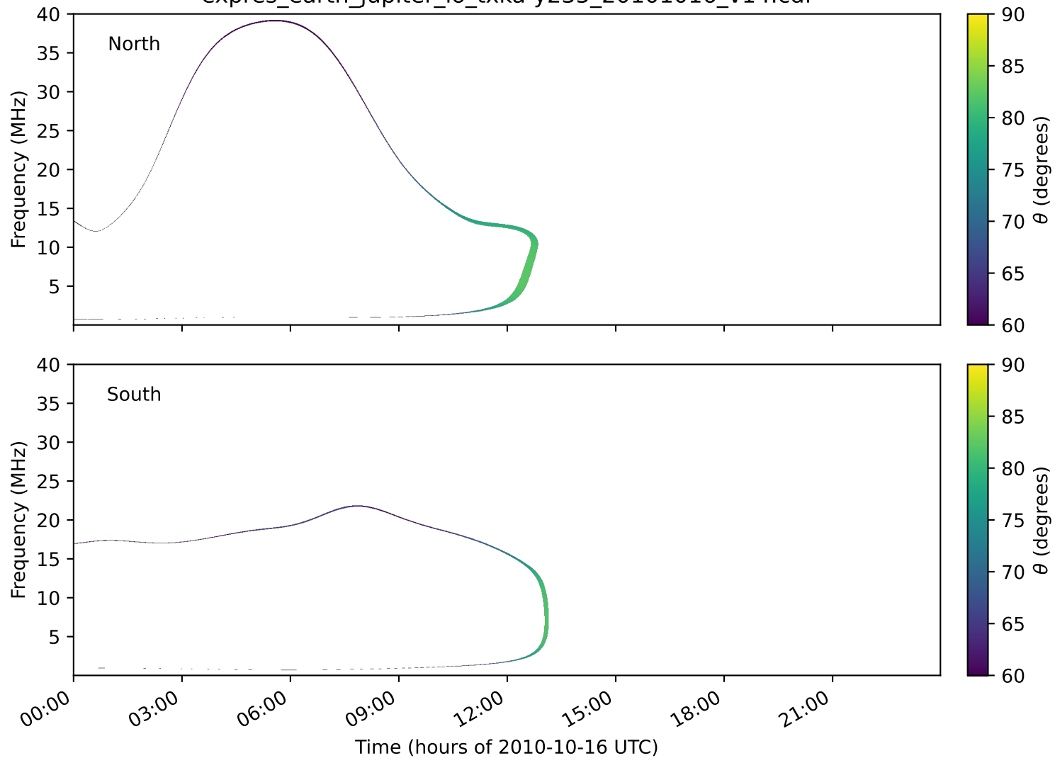
expres_earth_jupiter_io_txka-y235_20101016_v14.cdf
