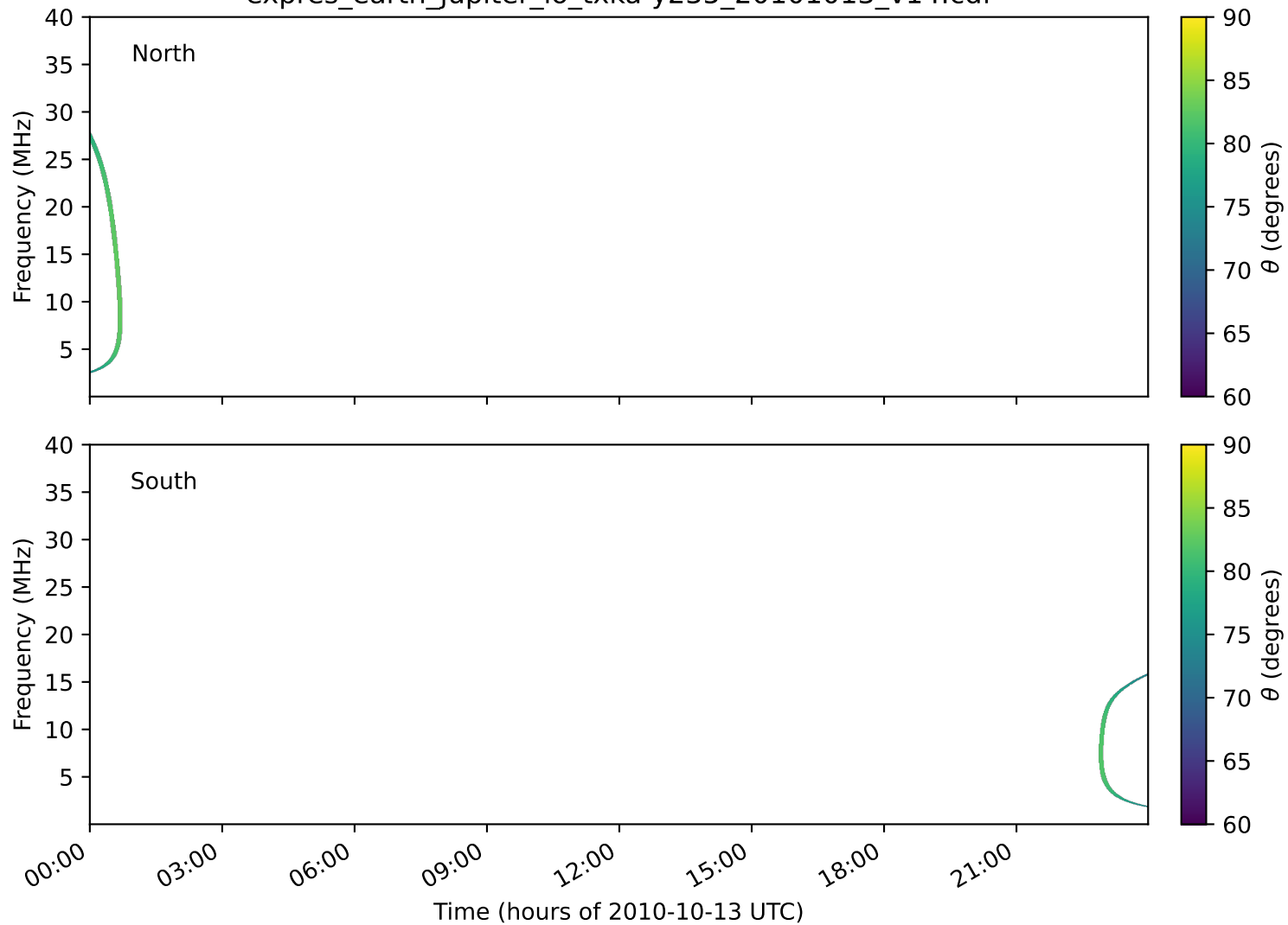
expres_earth_jupiter_io_txka-y235_20101013_v14.cdf
