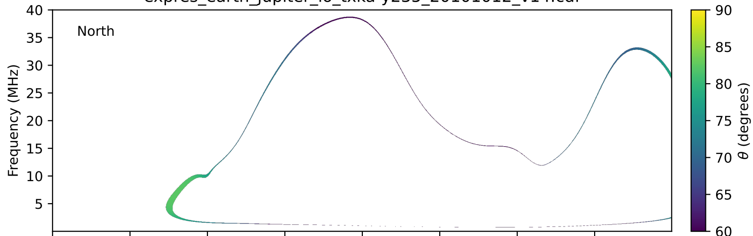
expres_earth_jupiter_io_txka-y235_20101012_v14.cdf
