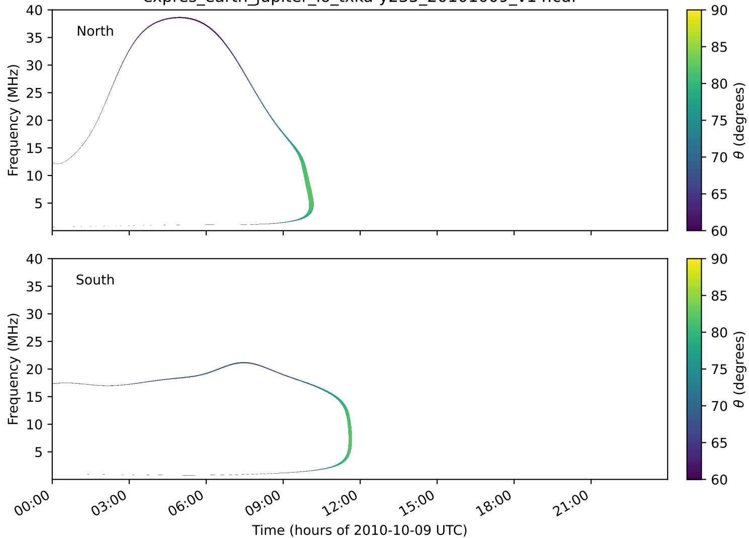
expres_earth_jupiter_io_txka-y235_20101009_v14.cdf
