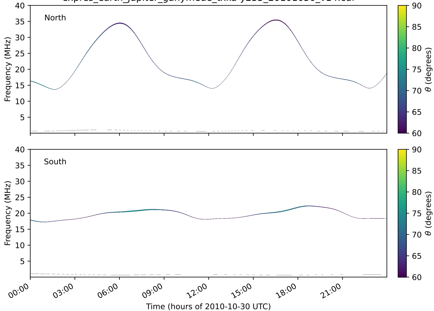
expres_earth_jupiter_ganymede_txka-y235_20101030_v14.cdf
