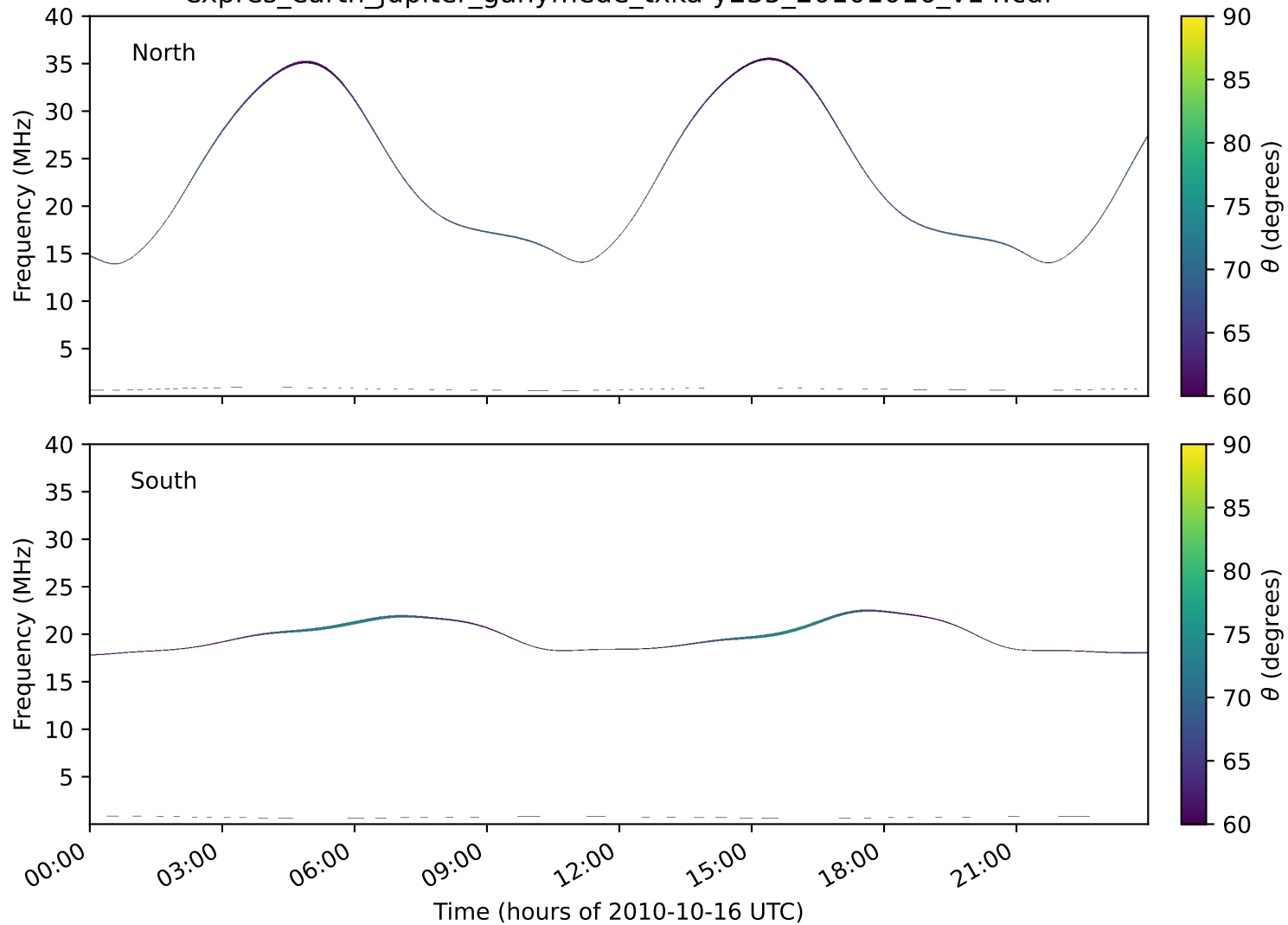
expres_earth_jupiter_ganymede_txka-y235_20101016_v14.cdf
