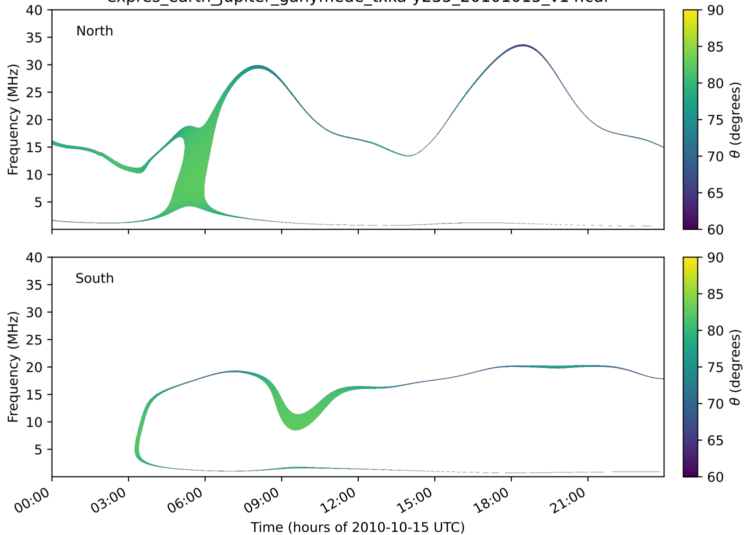
expres_earth_jupiter_ganymede_txka-y235_20101015_v14.cdf
